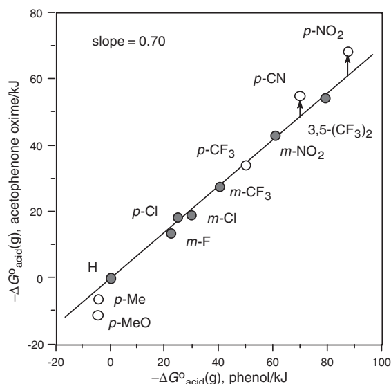
Figure 2. Plot of gas-phase acidities, acetophenone oximes vs. phenols. 19
