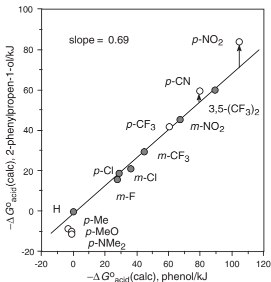
Figure 3. Plot of calculated acidities, 2-phenylpropen-1-ols vs. phenols.
