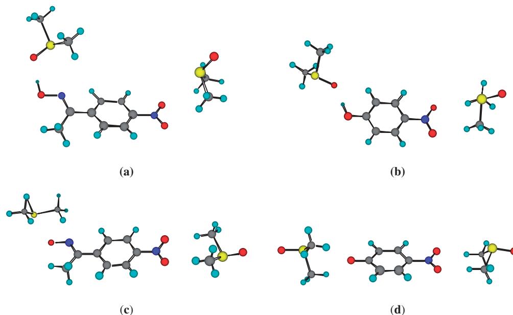
Chart 2. Optimized structures of complexes associated with two DMSO molecules. (a) p -Nitroacetophenone oxime, (b) p -nitrophenol, (c) p -nitroacetophenone oximate, and (d) p -nitrophenoxide.
