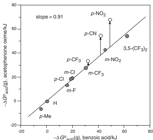
Figure 1. Plot of gas-phase acidities of acetophenone oximes against the corresponding benzoic acids. 22
