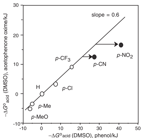
Figure 5. Plot of acidities in DMSO, acetophenone oximes vs. phenols.
