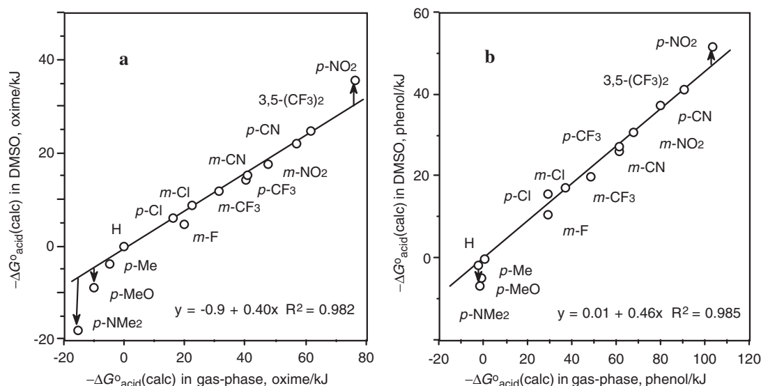
Figure 6. Comparison of calculated acidities between gas phase and DMSO (SCRF-PCM) for acetophenone oximes (a) and phenols (b).
