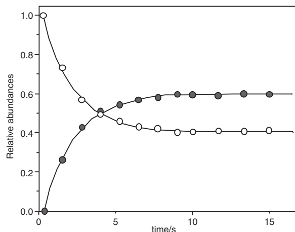
Figure 7. Time profile of anions formed from the binary mixture of m -CF 3 C 6 H 4 C(CH 3 )=NOH ( 1.61 \times 10^{-7} Torr) and o -FC 6 H 4 OH ( 2.27 \times 10^{-7} Torr). Closed circles; m/z 111 ( o -FC 6 H 4 OH), open circles; m/z 202 ( m -CF 3 C 6 H 4 C(CH 3 )=NOH).
