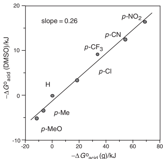
Figure 4. Plot of acidities of acetophenone oximes, DMSO vs. gas phase.
